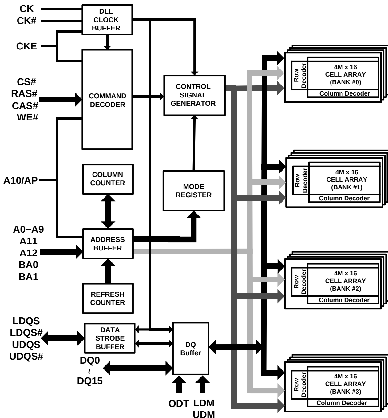
Figure 2. Block Diagram
