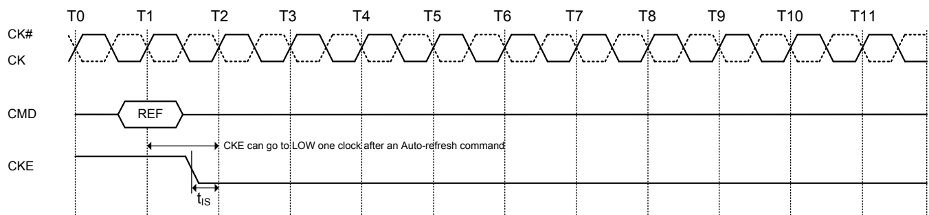
Figure 41. Refresh command to power-down entry
